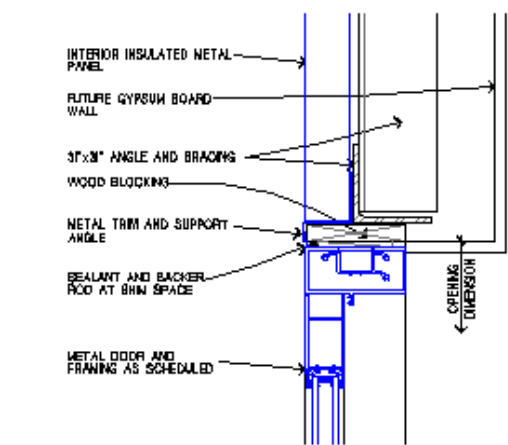
2 ALTERNATE BID #2 DOOR HEAD SCALE 3/4"=1'-0" 08400-64
