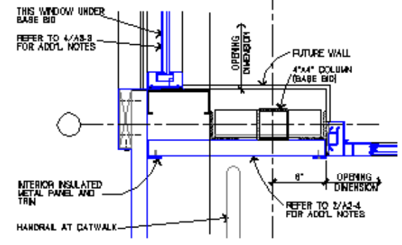
3 ALTERNATE BID #2 PLAN DETAIL SCALE 1 1/2"=1'-0" 08400-65
